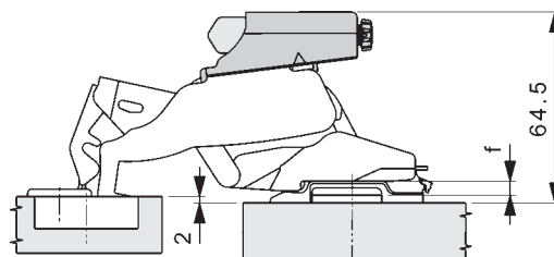
Soft-close® F65 with CS 65 hinge
