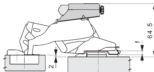
Soft-close® F65 with CST 65 hinge
